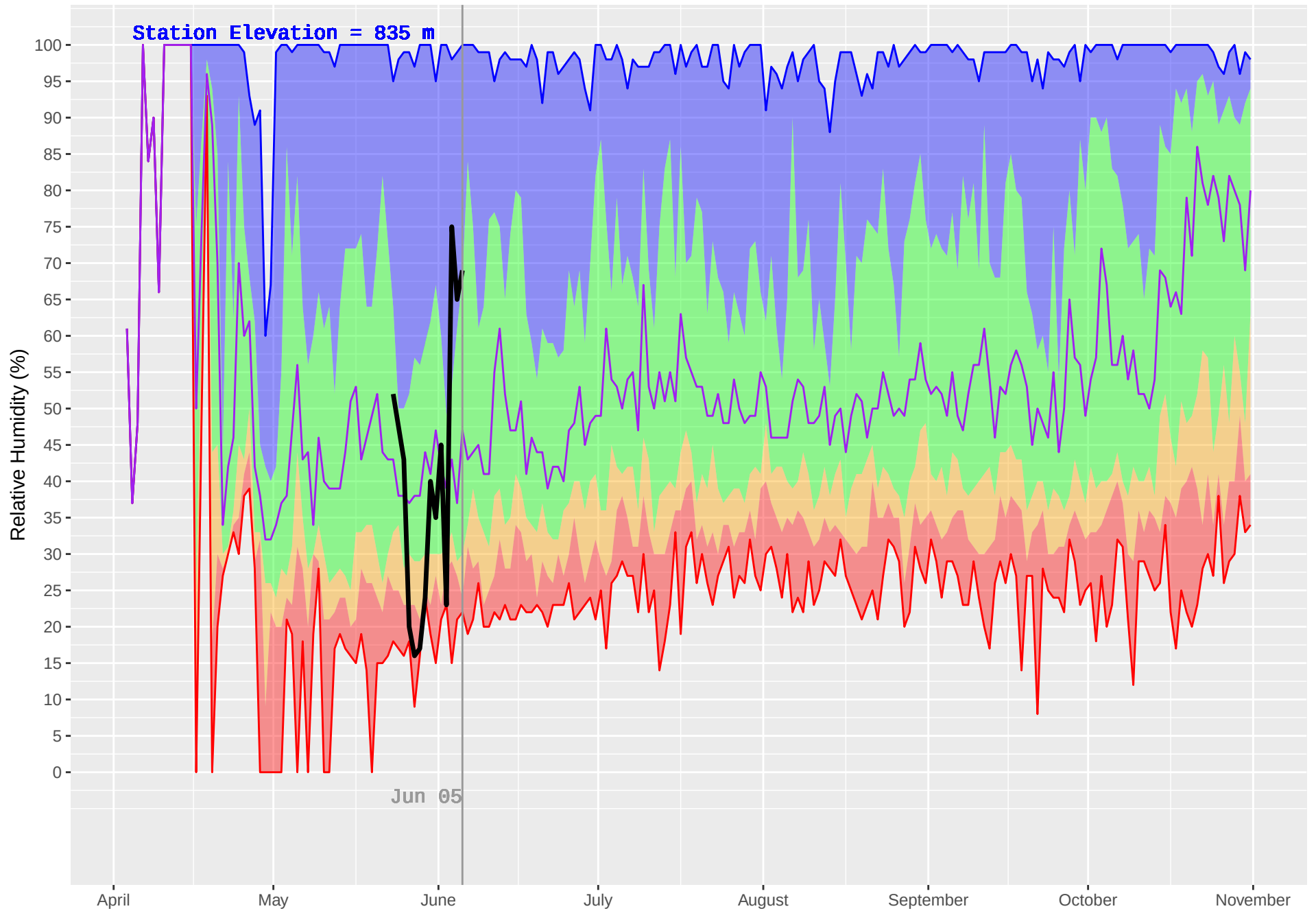
SILVER (120) : Historical (1986–2018) and Current (2019) Daily Relative Humidity
