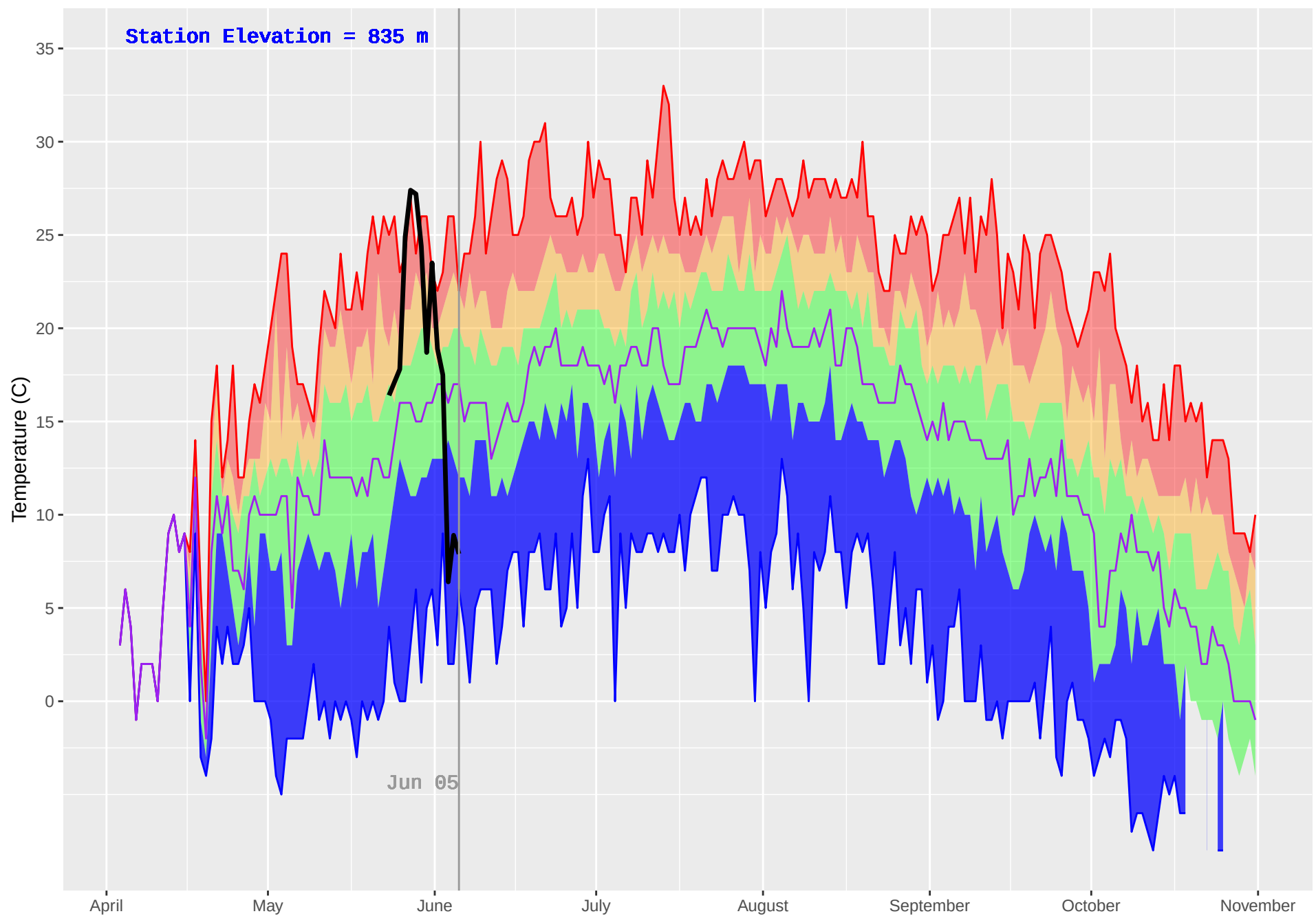
SILVER (120) : Historical (1986–2018) and Current (2019) Daily Temperature
