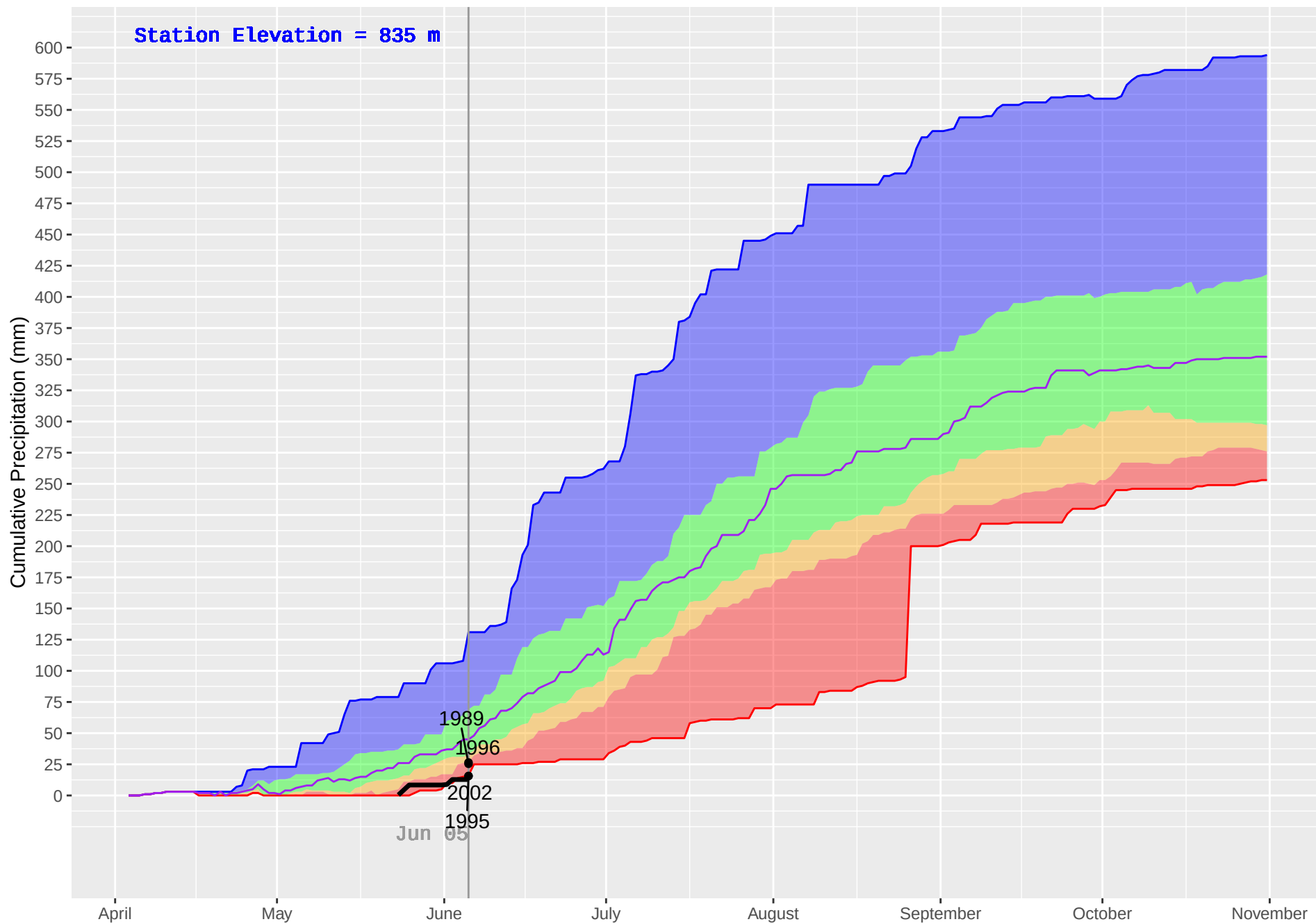
SILVER (120) : Historical (1986–2018), Current (2019) Daily Cumulative Precipitation
