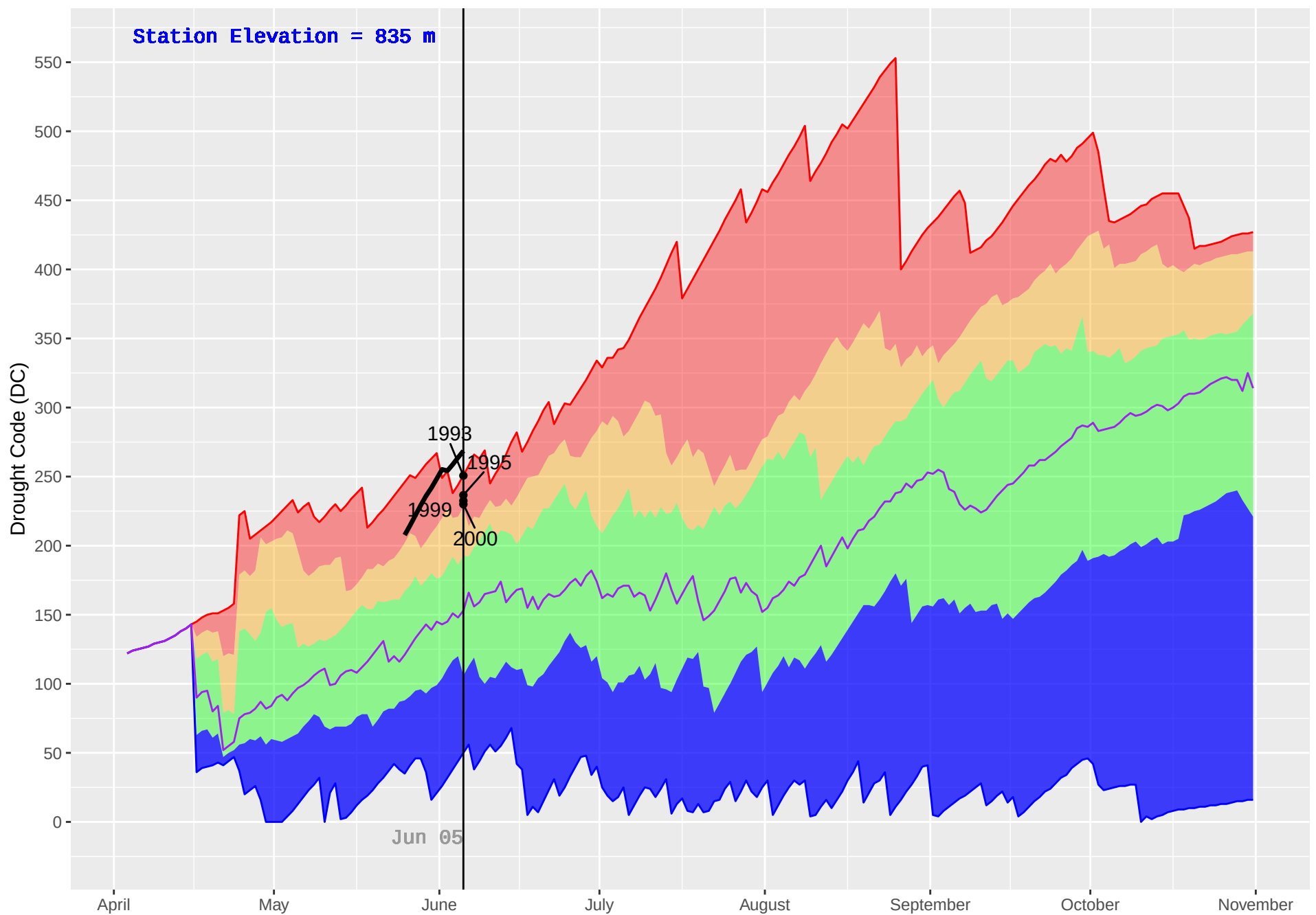
SILVER (120) : Historical (1986–2018) and Current (2019) Daily Drought Code (DC)
