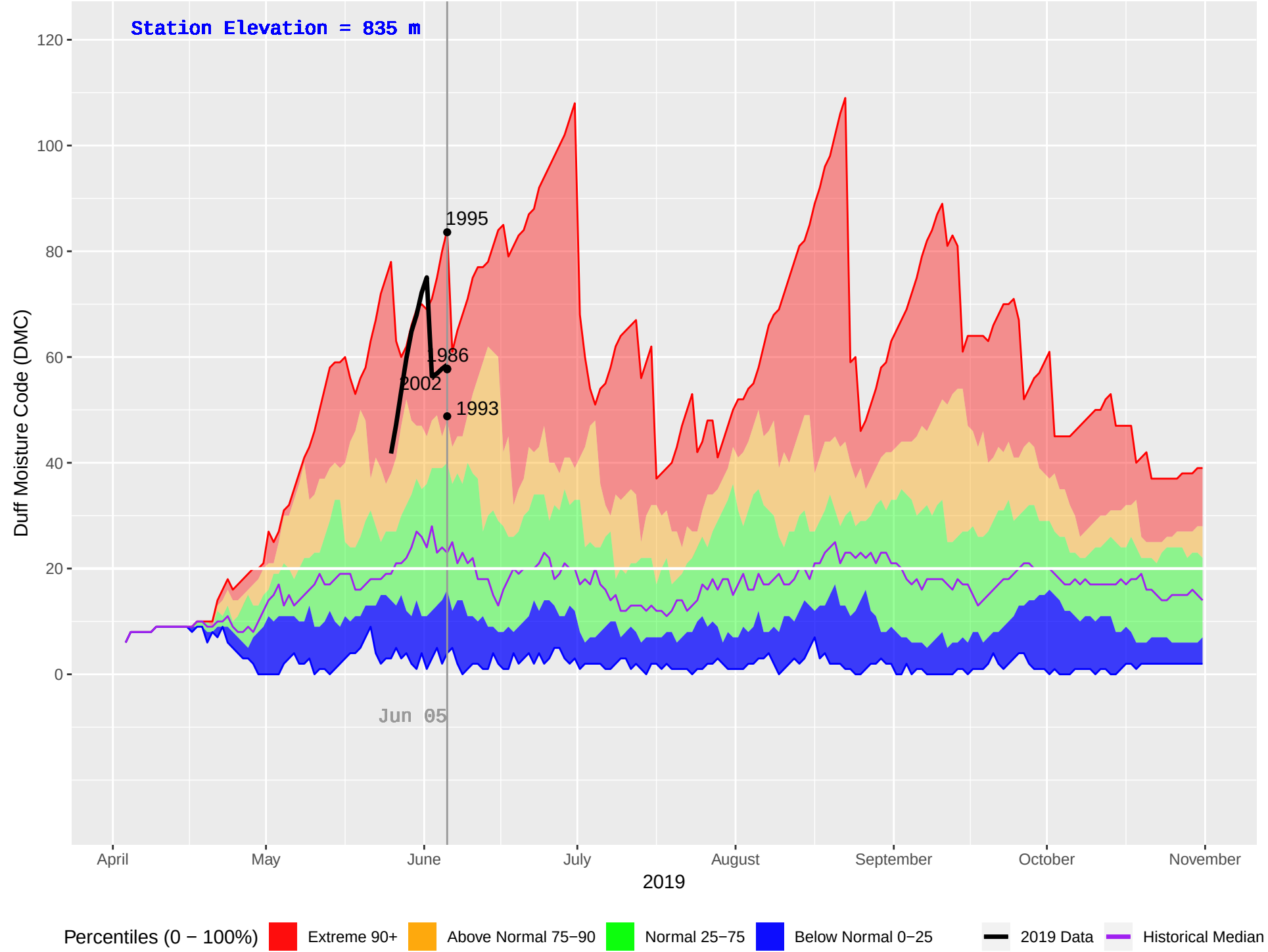
SILVER (120) : Historical (1986–2018), Current (2019) Daily Duff Moisture Code (DMC)
